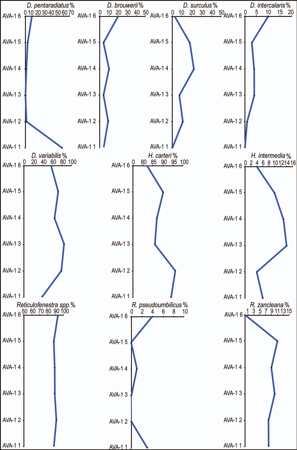
Appendix 3. Plots of the calcareous nannofossils frequencies.
